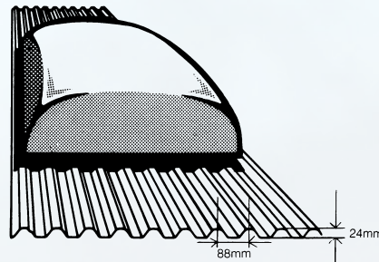
Spankdek (SD) 400mm - 600mm 1000mm - 1200mm
