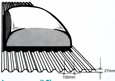
Longspan (LS) 600mm - 1200mm
