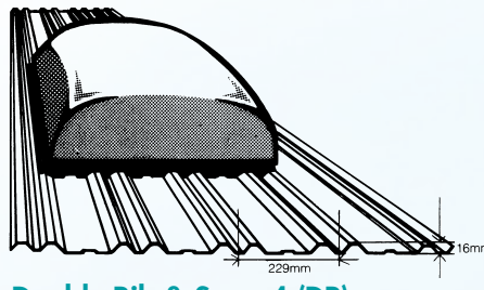
Double Rib & Span 4 (DR) 600mm
